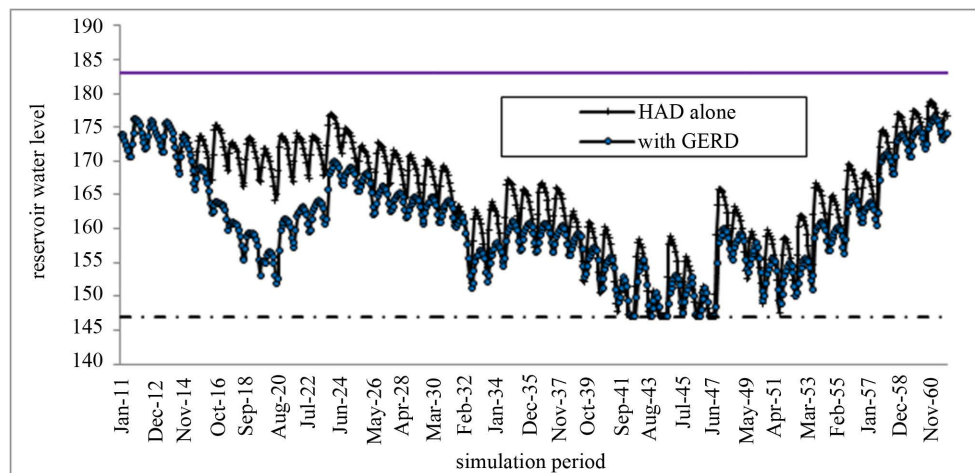
Figure 9. HAD reservoir water level during filling and operation phases of GERD.
